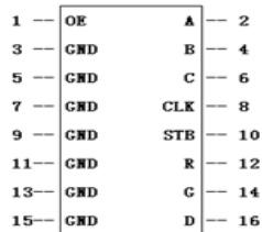
HUB12 Port
