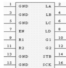
HUB08 Port
